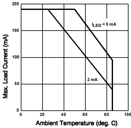
Figure 1. Typical Current Derating Curve
